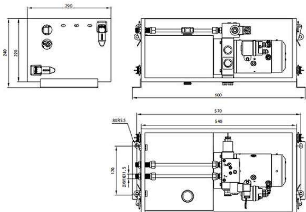
Outline Dimension
